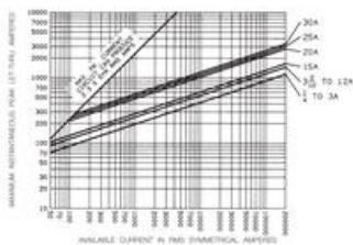
Peak Let-Thru Current Data - ATDR 1/4 till 30, 600 Volts AC
