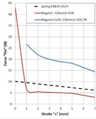
Force-stroke curve(F-S)
