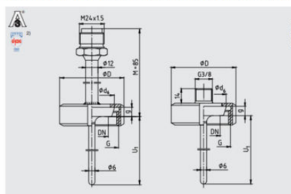
Union nut process connection DIN 11851 with conical coupling (milk thread fitting)
